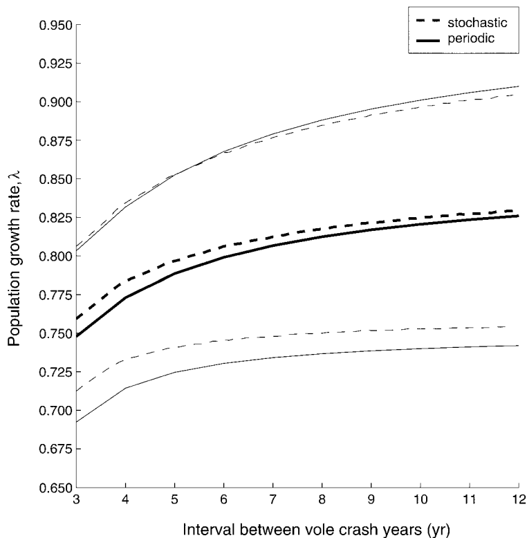
FIG. 4. Population growth rate for the periodic model \lambda_{pd} ; heavy solid line) and stochastic model ( \lambda_s ; heavy dashed line) as a function of the interval between vole crash years. Light lines indicate \pm SE from bootstrap estimates of population growth rate.
