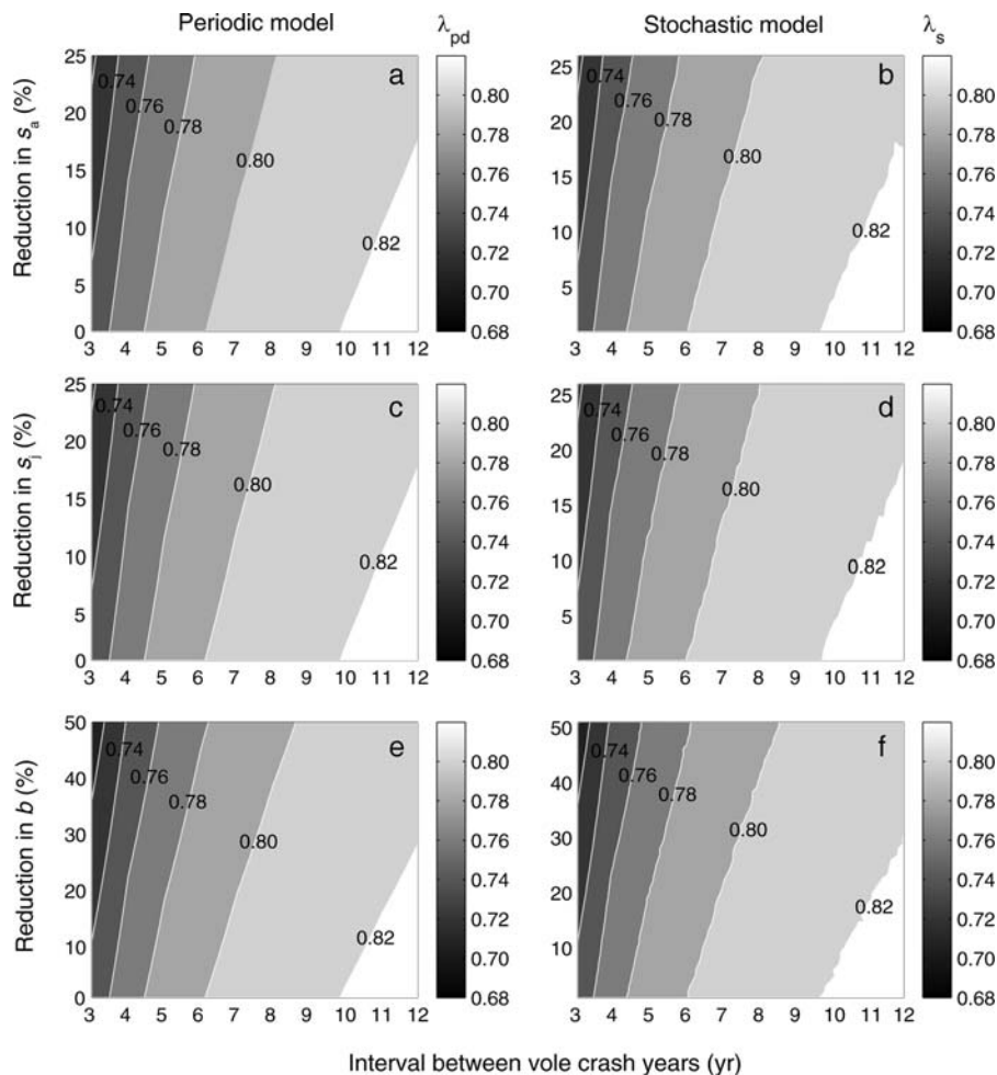
FIG. 5. Population growth rate for the periodic model ( \lambda_{pd} ; left-hand panels) and stochastic model ( \lambda_s ; right-hand panels) as a function of the interval between vole crash years and percentage reduction in (a,b) apparent adult survival s_a , (c,d) apparent juvenile survival s_j , and (e,f) fecundity b . The white contour lines represent lines of equal population growth rate. The near vertical alignment of these contours demonstrates the small response of \lambda_{pd} and \lambda_s to parameter reductions. A greater change is seen along the x -axis, showing a greater response to changes in the frequency of vole crashes. Note the difference in scale on the y -axis for reductions in fecundity.
