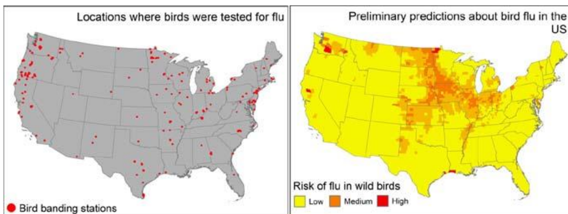
Figure 1. Sampling locations (left) and preliminary predictions of bird flu in wild birds (right) in the USA using data collected from MAPS sites.
